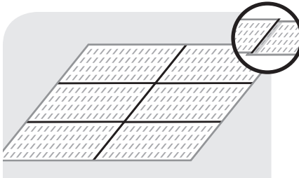
Overlap SimpleMat edges 1/8" to 1/4" (3 - 6 mm). Overlapping is shaded in illustration.
